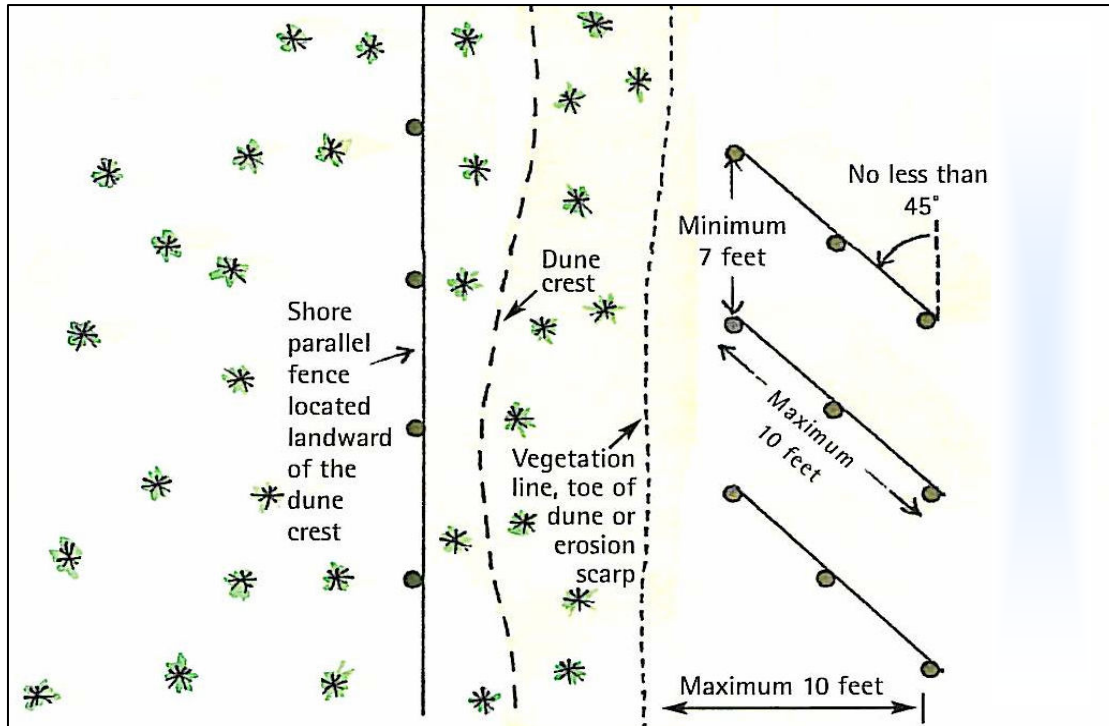
A. Example Sand Fence Installation
